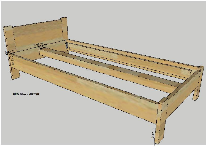
Figure 1: the dimension of the bed
