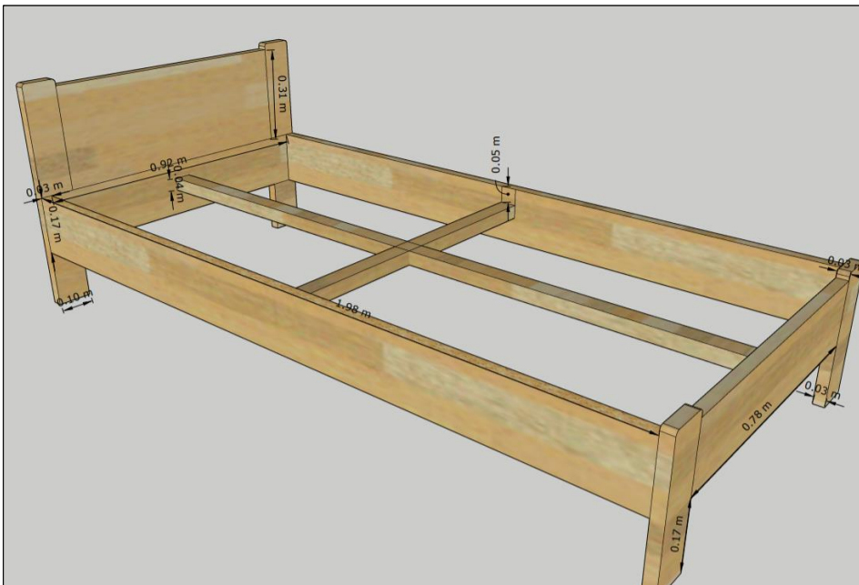
Figure 2; Bed Dimensions (Detailed)
